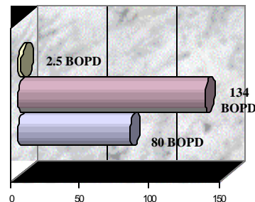
Misener Sandstone
